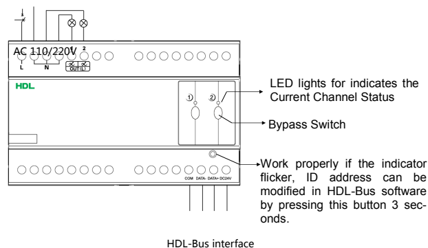
HDL-Bus Definition for cable
