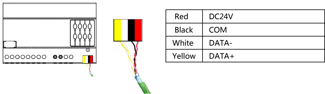
HDL-BUS Wiring Diagram
