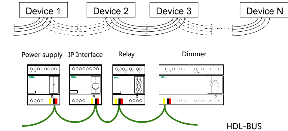
HDL-BUS Wiring Diagram
